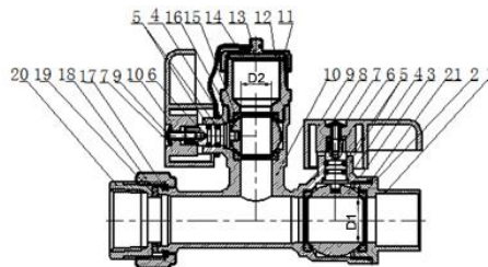
Cold Water Valve
