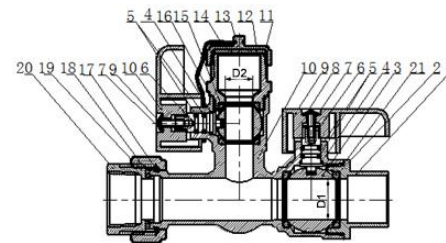
Hot Water Valve
