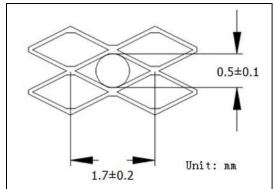
Stainless Steel Screen #20 mesh (0.85 mm) Diagram
